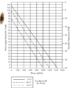
MODEL 331 PERFORMANCE
