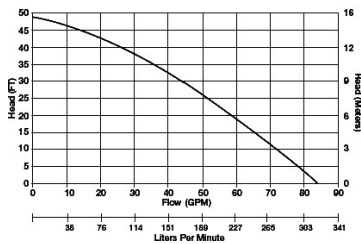
Performance Curve: 290-Series
