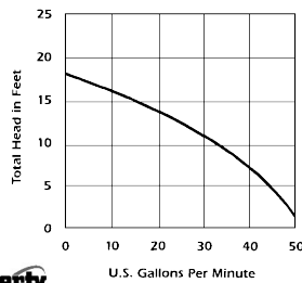
PERFORMANCE CURVE
