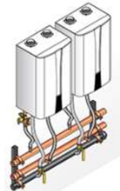
2-side-by-side wall kit installed
