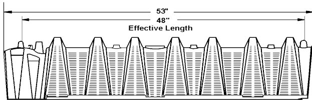
Quick4 Equalizer 36 Chamber - Side View
