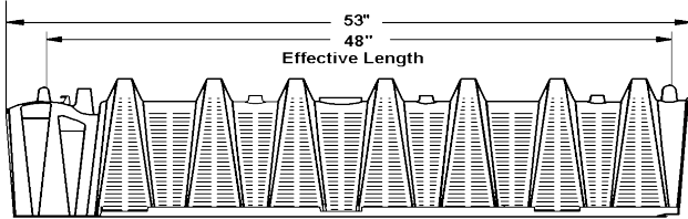
Quick4 Equalizer 36 Chamber - Side View
